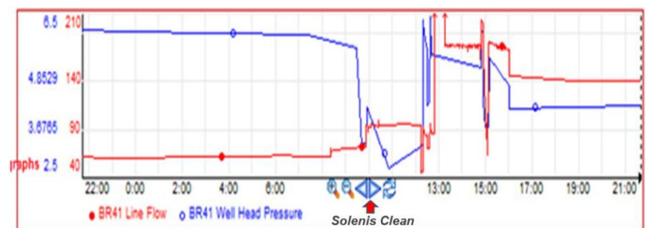
Flow and pressure graph of the reinjection well before and after implementation of GeoSol well cleaning program.
